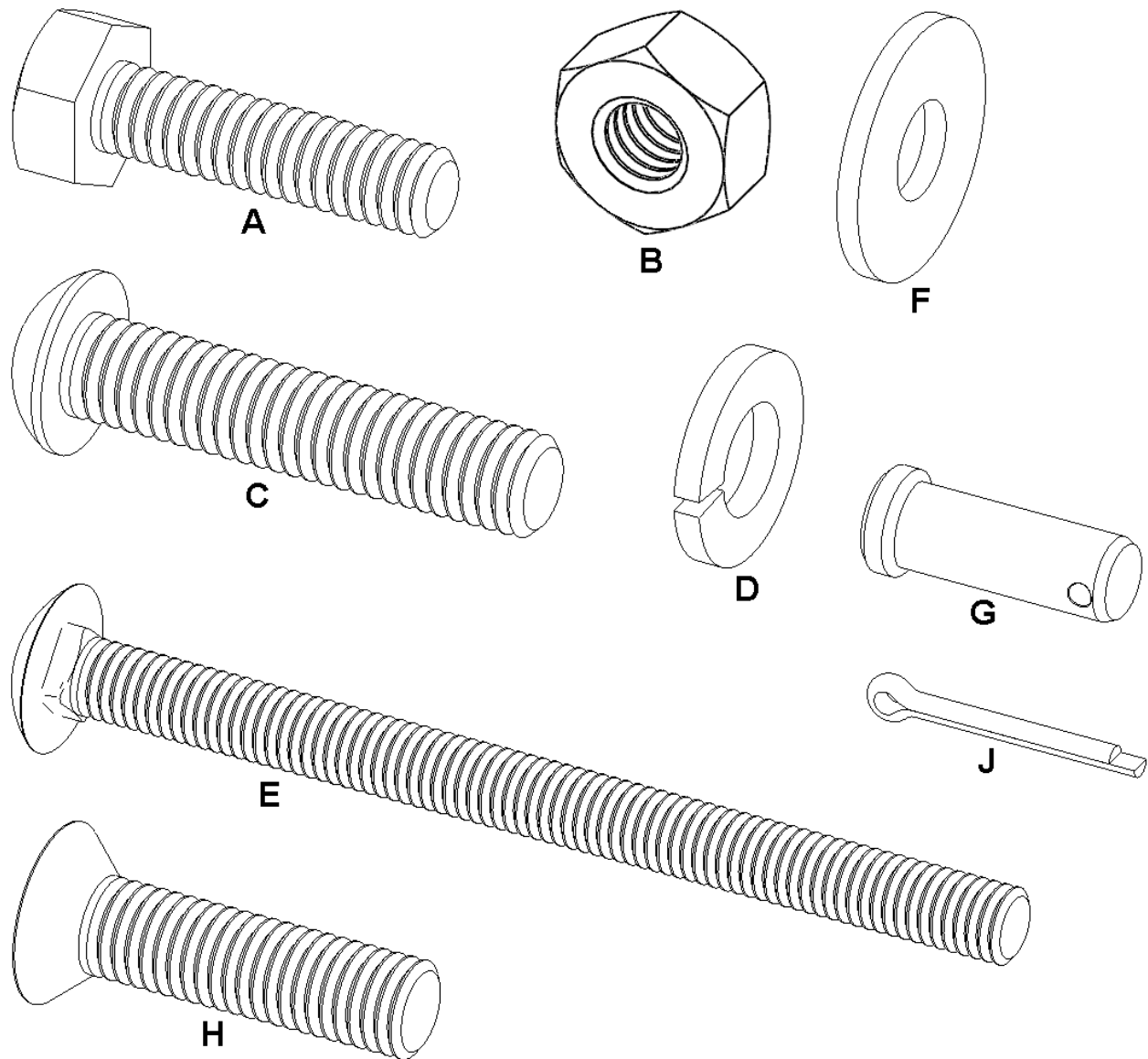
Figure 11.1: Fasteners
