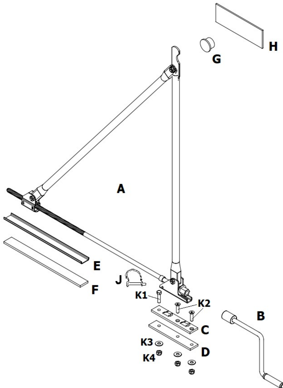
Figure 9.1: Double Hook Rear Brace (2025 +)
