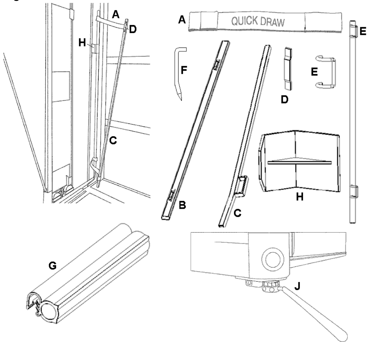
Figure 6.3: Headboard Parts
