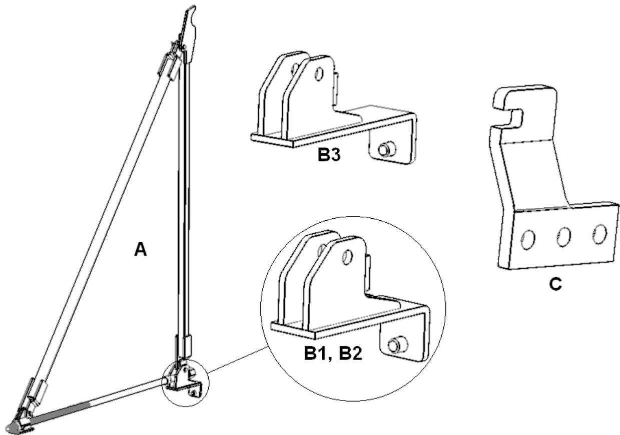
Figure 9.5: Single Hook Rear Braces (1997 - 2005)
