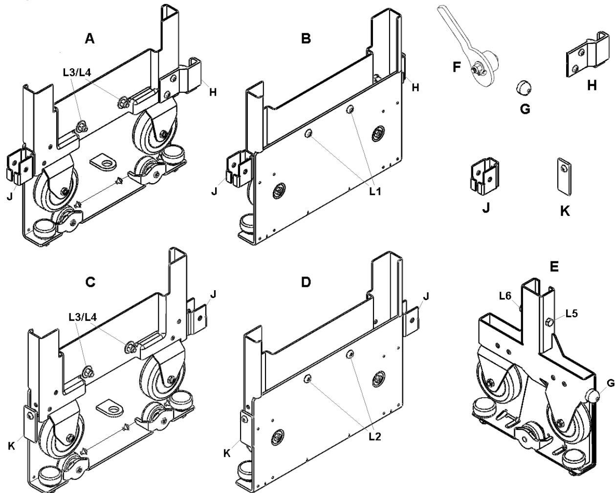
Figure 5.1: Carriers
