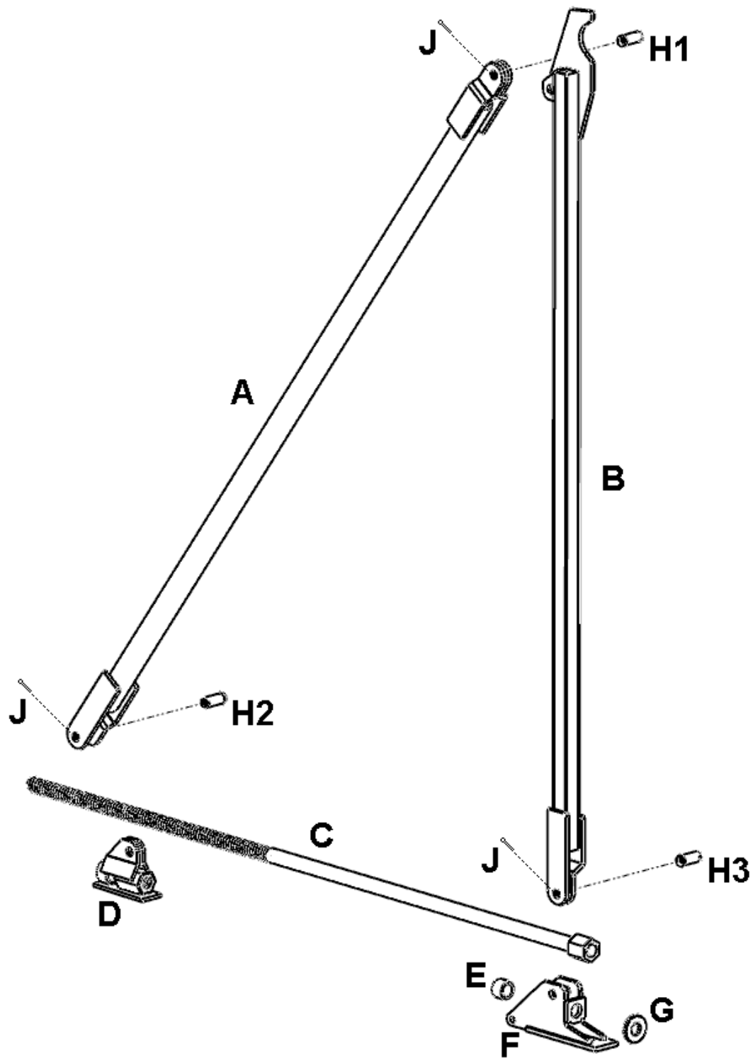
Figure 9.4: Double Hook Rear Brace Sub-parts (2006 - 2025)
