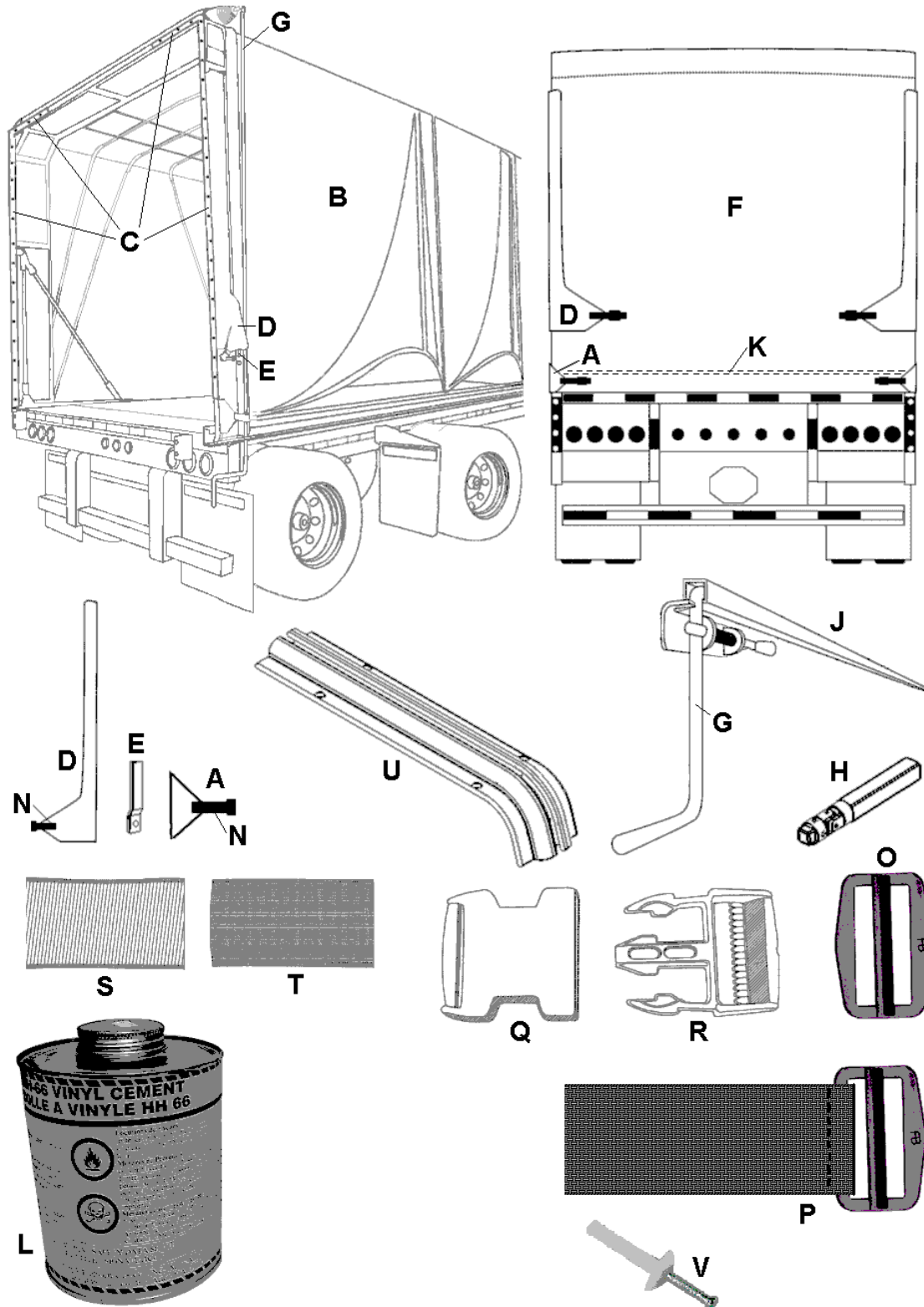
Figure 2.1: Vinyl Tarp
