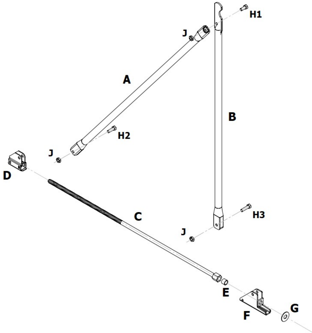
Figure 9.2: Double Hook Rear Braces (2025 +)
