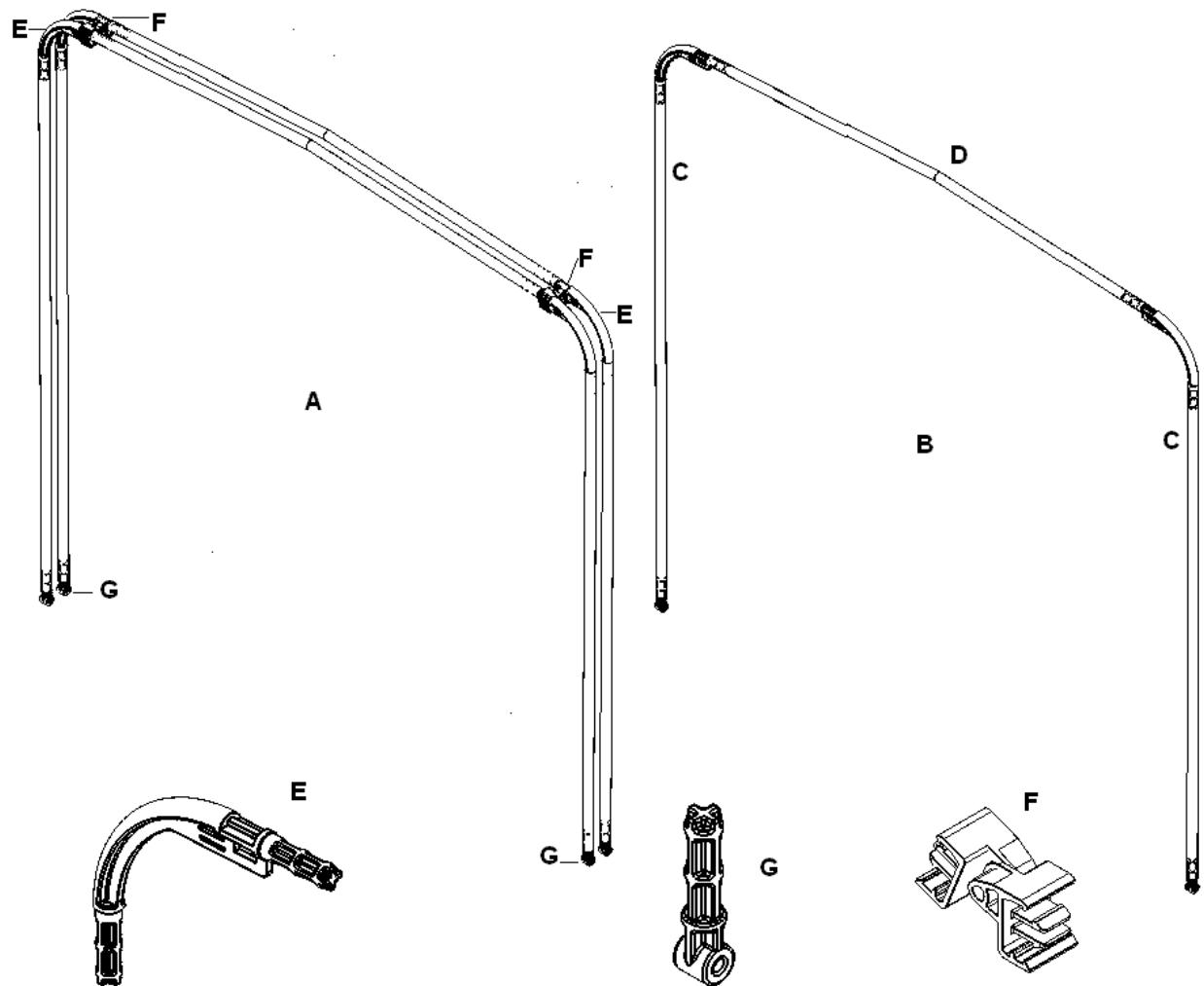
Figure 8.1: Lifter Bows
