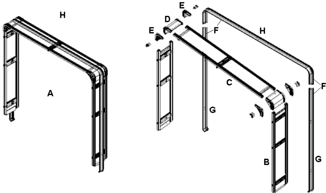
Figure 7.5: Rear Bows
